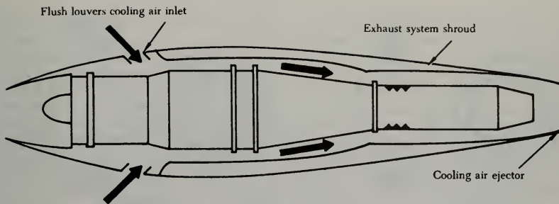
FIGURE 1-65. Exhaust system shroud.
